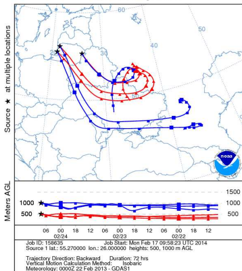
NOAA HYSPLIT MODEL Backward trajectories ending at 0800 UTC 24 Feb 13 GDAS Meteorological Data
