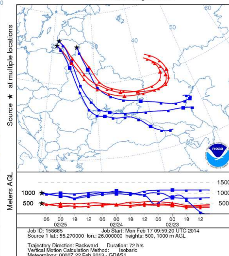
NOAA HYSPLIT MODEL Backward trajectories ending at 0800 UTC 25 Feb 13 GDAS Meteorological Data
