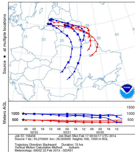
NOAA HYSPLIT MODEL Backward trajectories ending at 0800 UTC 22 Feb 13 GDAS Meteorological Data
