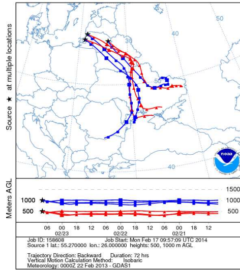
NOAA HYSPLIT MODEL Backward trajectories ending at 0800 UTC 23 Feb 13 GDAS Meteorological Data
